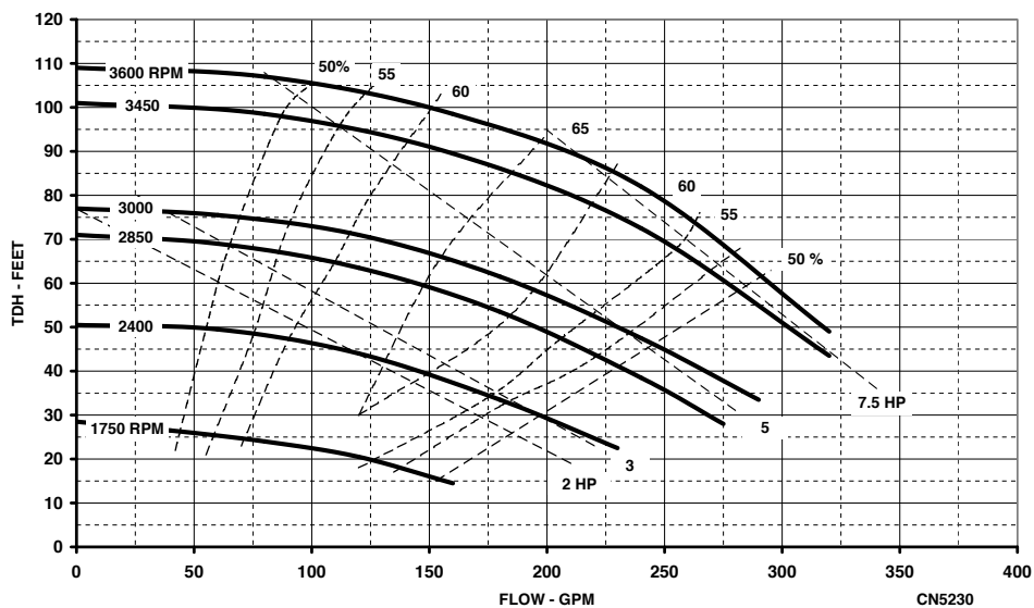
SERIES 200 5.44 "C" Impeller
