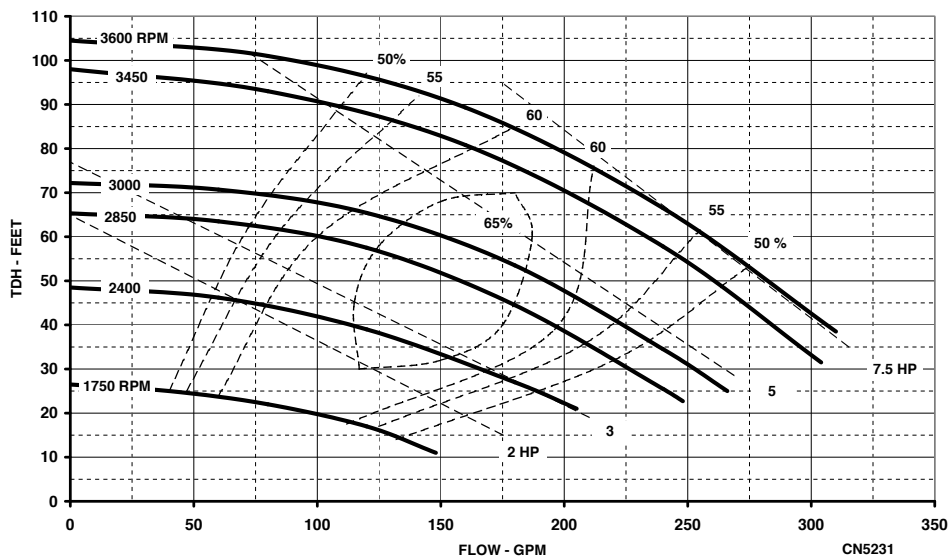
SERIES 200 5.4 "B" Impeller
